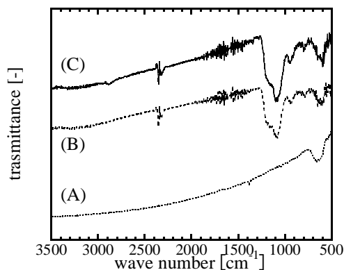
Fig. 1 FI-IR spectra of particles.
